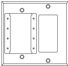
IPS-WP2D 1 IPS & 1 Decora Opening
