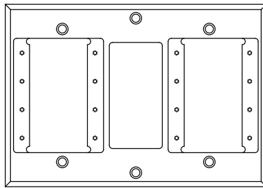
IPS-WP2T 2 IPS & 1 Decora Opening
