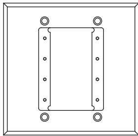
IPS-WP1D 1 IPS Opening
