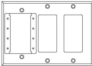
IPS-WP3T 1 IPS & 2 Decora Openings
